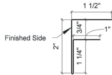
F-channel
