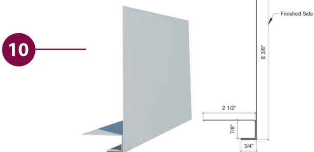
Overhead Door Trim w/J-channel
