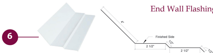
Side Wall Flashing
